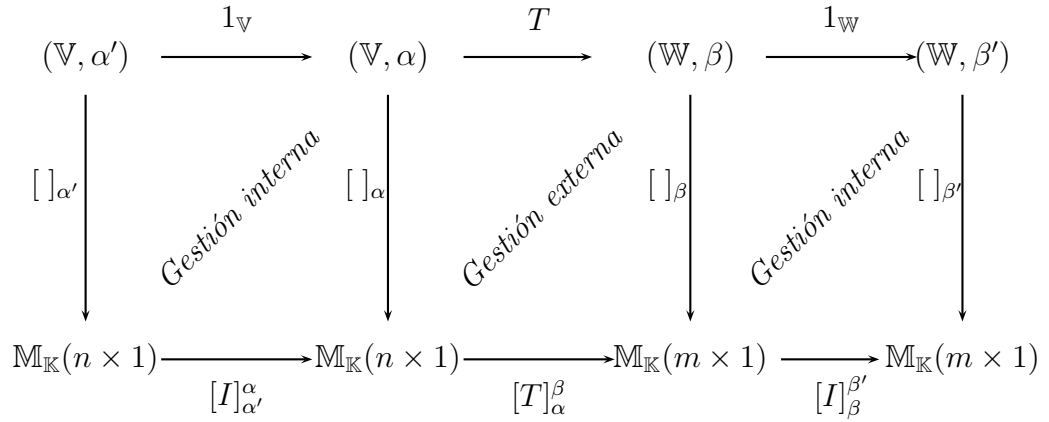
Figura 6: [T]_{\alpha'}^{\beta'} = [I]_{\beta}^{\beta'} \cdot [T]_{\alpha}^{\beta} \cdot [I]_{\alpha'}^{\alpha}
