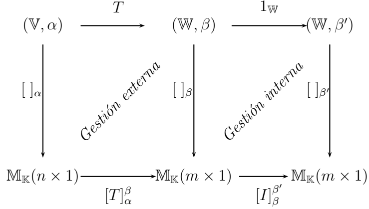
Figura 5: [T]_{\alpha}^{\beta'} = [I]_{\beta}^{\beta'} \cdot [T]_{\alpha}^{\beta}
